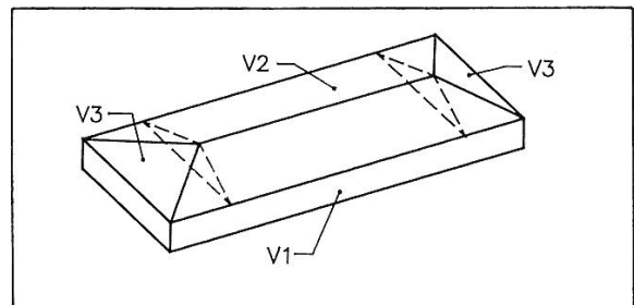
Fig 4-3. The three grain volumes of a flat storage.
